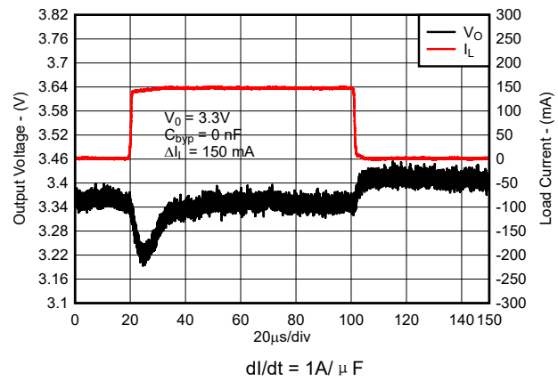
图 7-13. Load Transient Response (New Chip)
