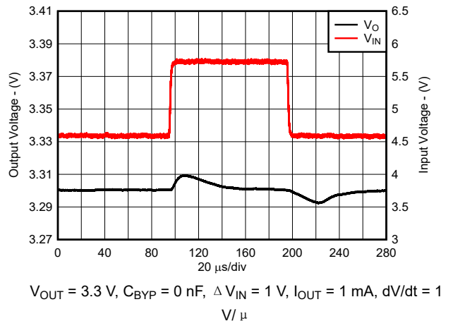
图 8-14. Line Transient Response for New Chip
