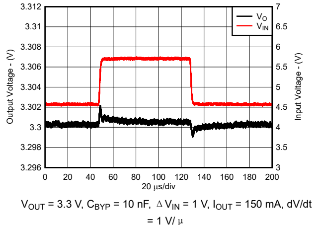
图 8-12. Line Transient Response for New Chip
