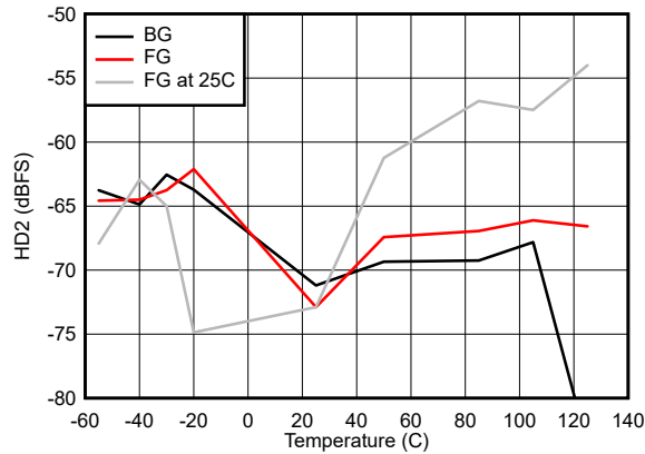
Low Power Mode, F_{IN} = 347 MHz
