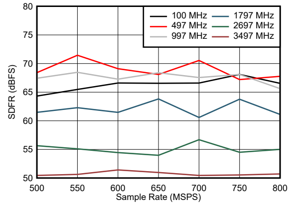
图 7-20. SFDR vs Sample Rate
