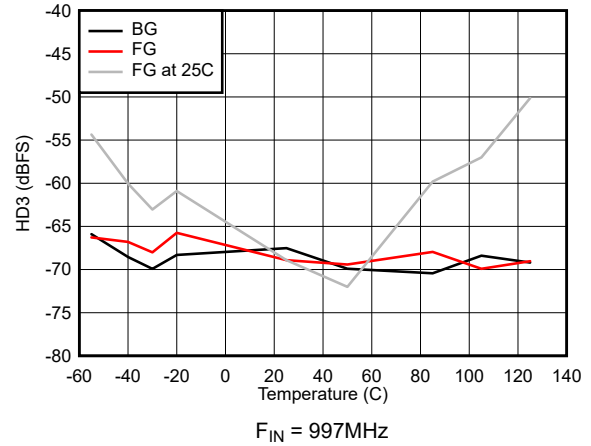
图 7-38. HD3 vs Temperature
