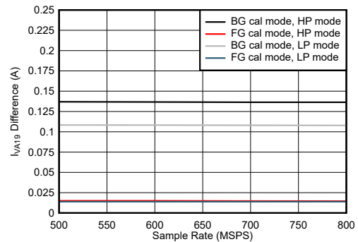
图 7-106. Single Channel, I_{VA19} Change with Calibration Mode
