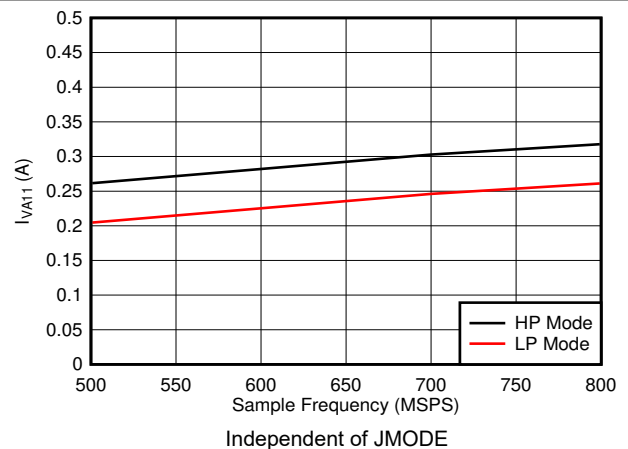
图 7-96. Single Channel, I_{VA11} vs F_S
