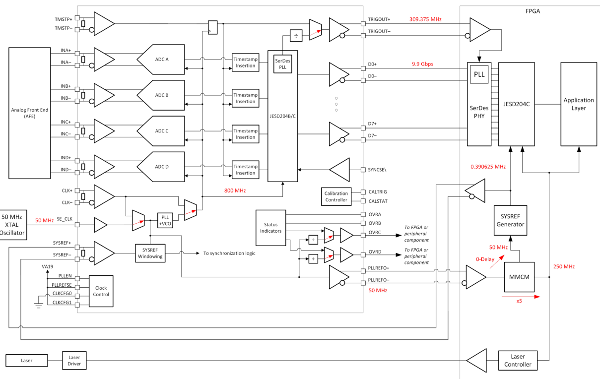
图 9-1. Typical Configuration for a LiDAR Digitizer
