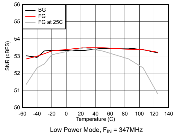
图 7-40. SNR vs Temperature
