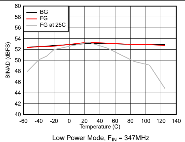
图 7-42. SINAD vs Temperature
