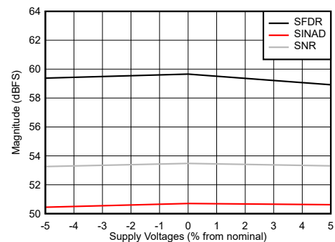
Low Power Mode, F_{IN} = 347 MHz
