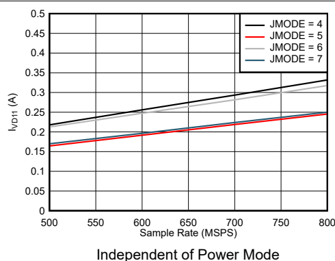
图 7-78. Quad Channel, I_{VD11} vs F_S for JMODES 4 - 7
