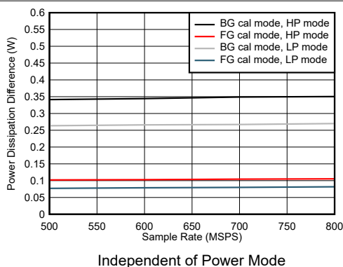
图 7-101. Quad Channel, Power Dissipation Change with Calibration Mode
