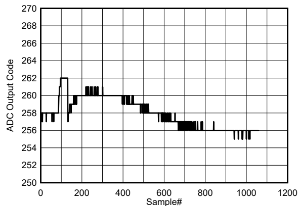
图 7-116. Background Core Transition (DC midscale input)
