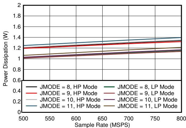
图 7-83. Dual Channel, Power Dissipation vs F_S for JMODES 8 - 11
