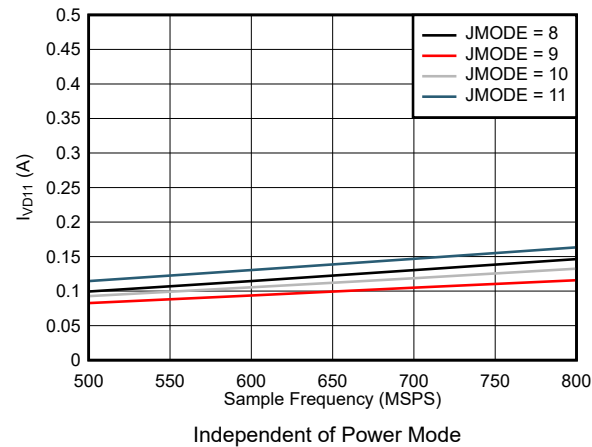
图 7-99. Single Channel, I_{VD11} vs F_S for JMODES 8 - 11
