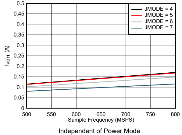
图 7-98. Single Channel, I_{VD11} vs F_S for JMODES 4 - 7
