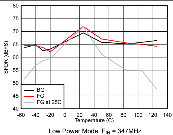
图 7-41. SFDR vs Temperature
