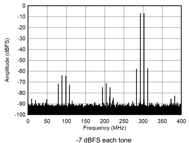
图 7-54. Single Tone FFT at 2698 MHz
