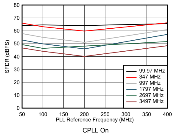
图 7-64. SFDR vs Reference Clock Frequency
