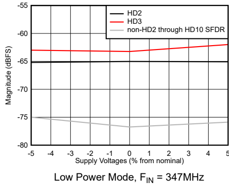
图 7-49. HD2, HD3 and Worst non-HD2/3 Spur vs Supply Voltage
