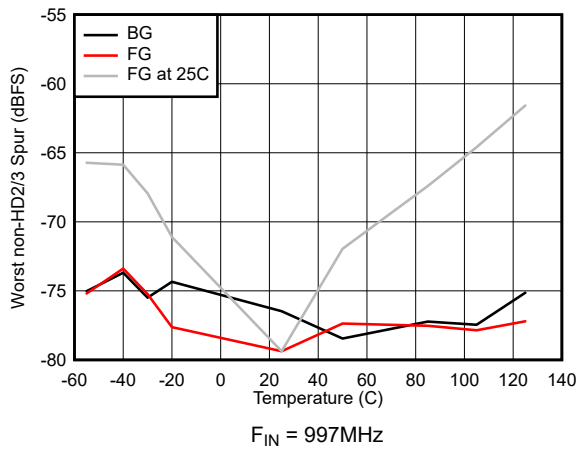
图 7-39. Worst non-HD2/3 Spur vs Temperature
