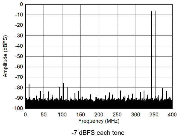
图 7-51. Single Tone FFT at 348 MHz
