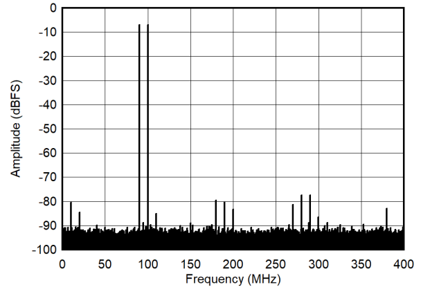
图 7-50. Single Tone FFT at 95 MHz
