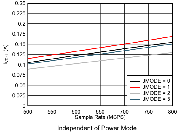
图 7-97. Single Channel, I_{VD11} vs F_S for JMODES 0 - 3
