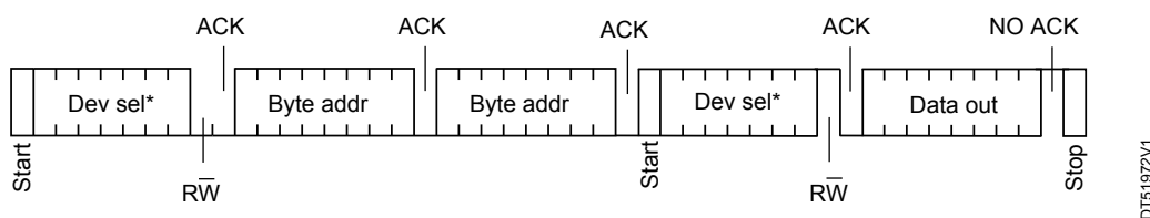
Figure 18. Random read DTI register
