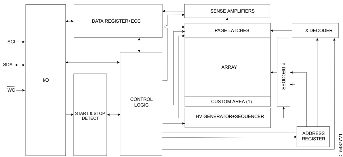
Figure 4. Block diagram
