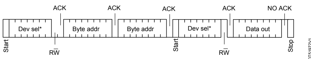
Figure 20. Random read SWP register
