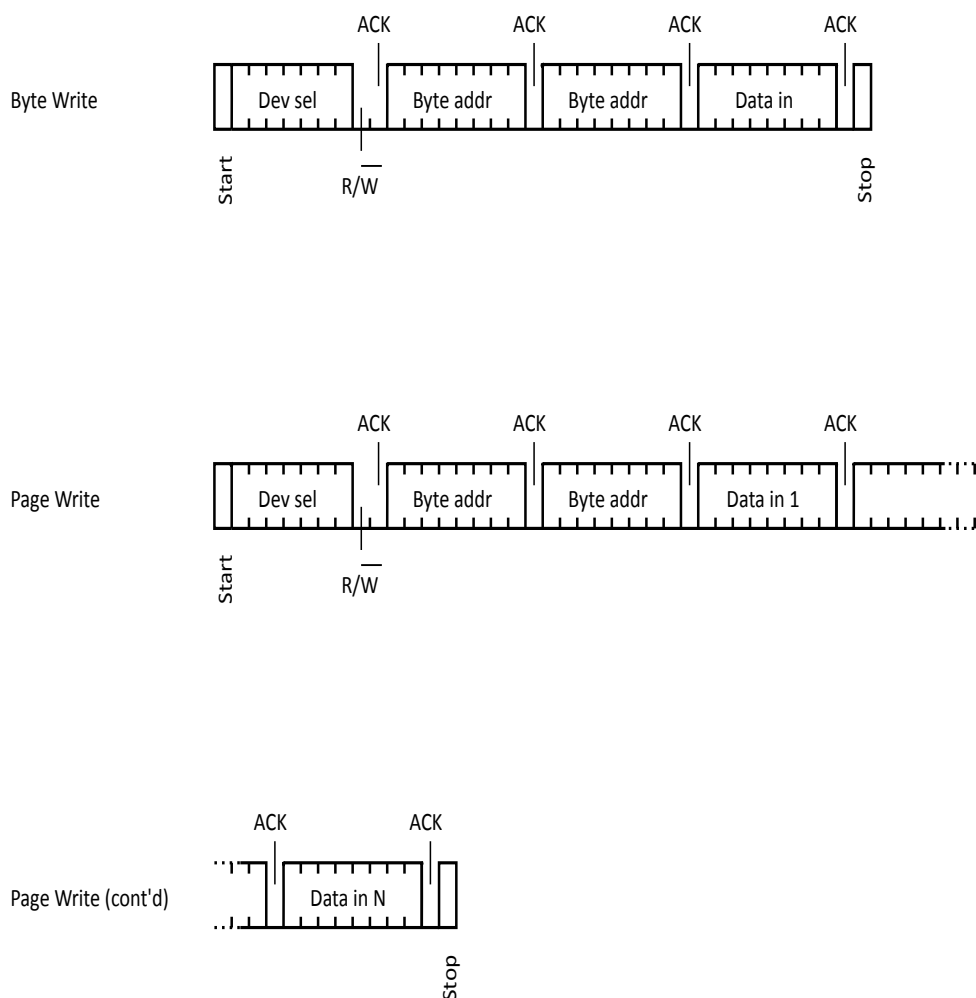
Figure 12. Write identification page (page unlocked)
