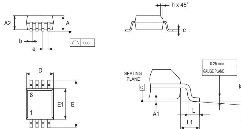
Figure 32. SO8N – Outline
