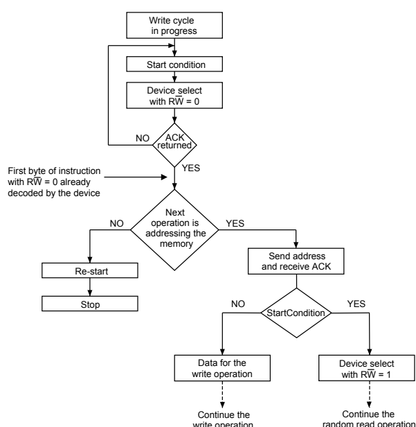
Figure 16. Write cycle polling flowchart using ACK
