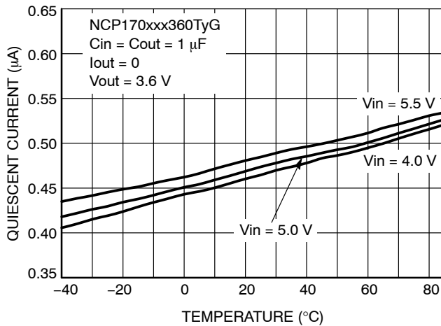
Figure 17. Quiescent Current vs. Temperature, V_{out} = 3.6 \text{ V}
