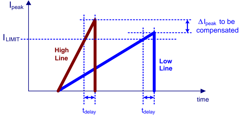
Figure 67. Needs for Line Compensation For True Overpower Protection
