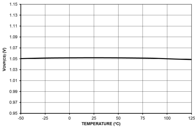
Figure 13. Over Voltage Protection Threshold at CS Pin V_{OVP(CS)}
