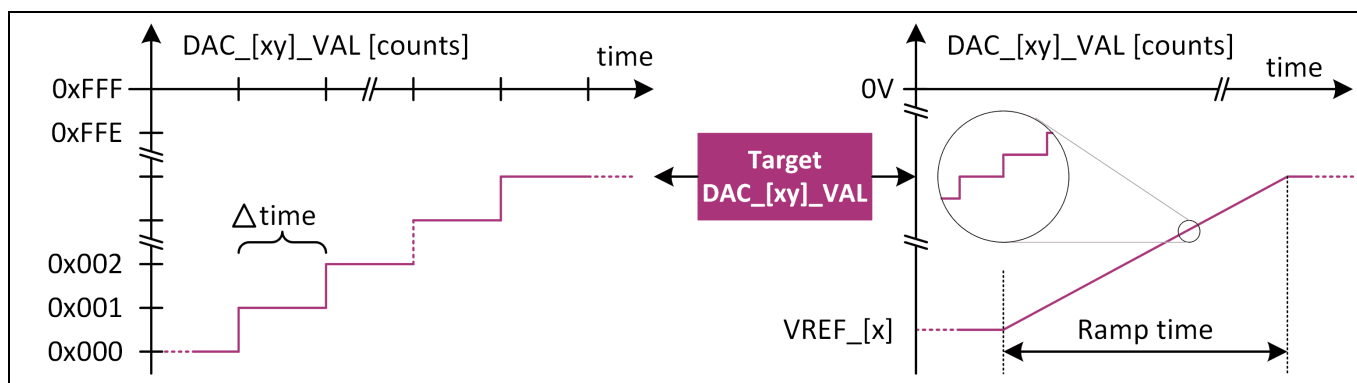
Figure 51 DAC Slope
