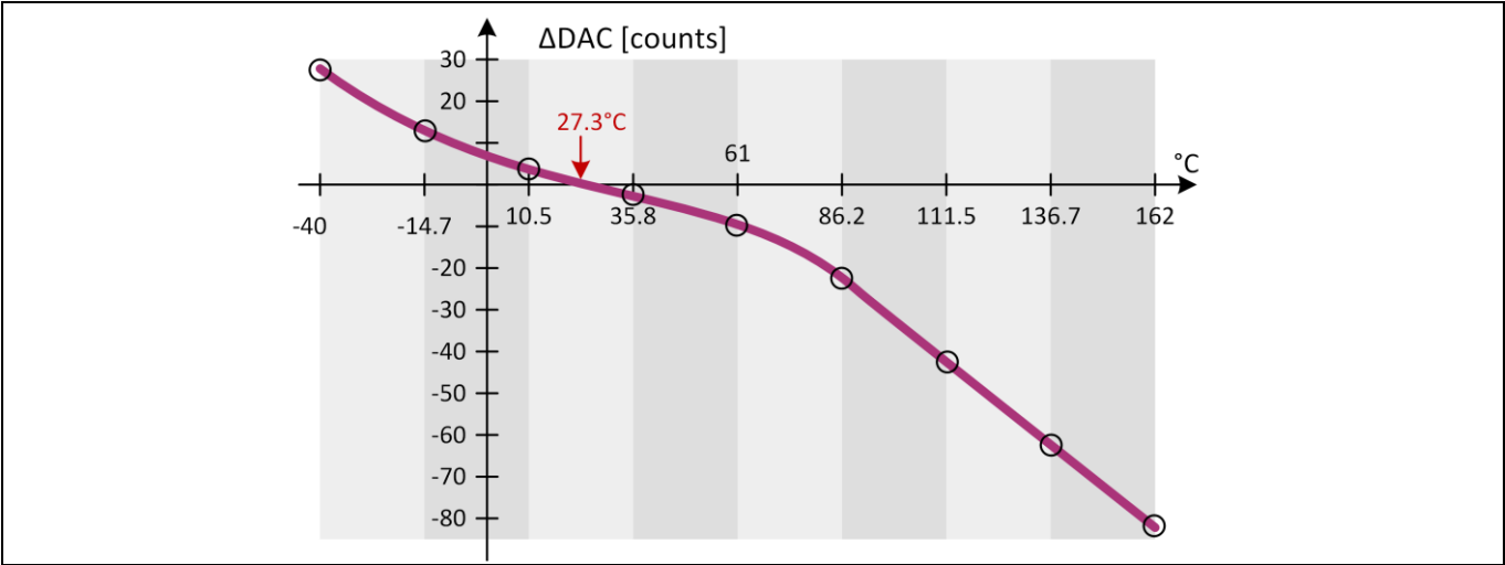
Figure 54 Delta DAC Over Temperature
