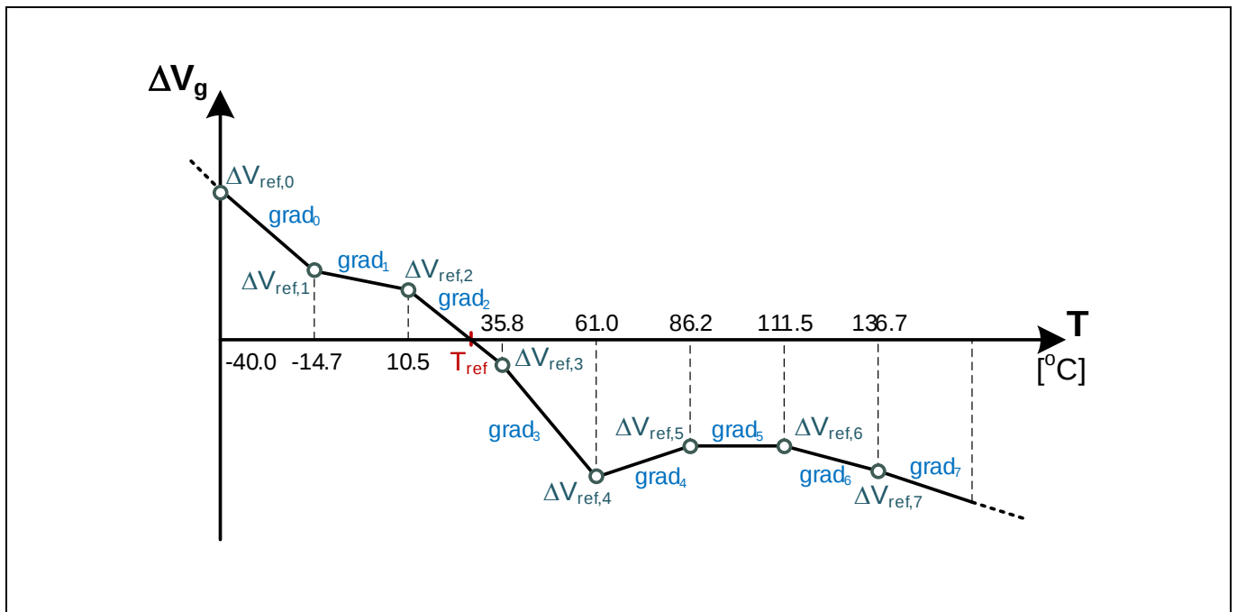
Figure 8 Coefficients in LUT for temperature compensation
