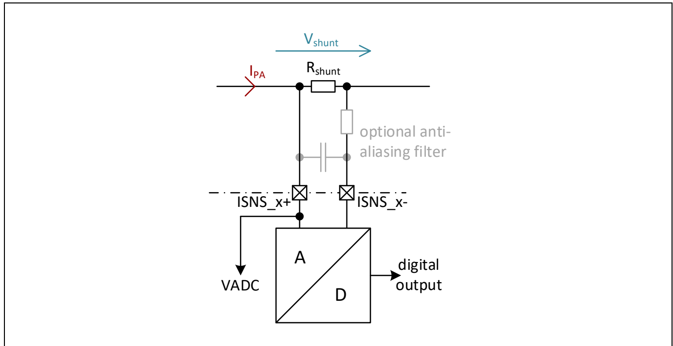
Figure 13 Shunt ADC
