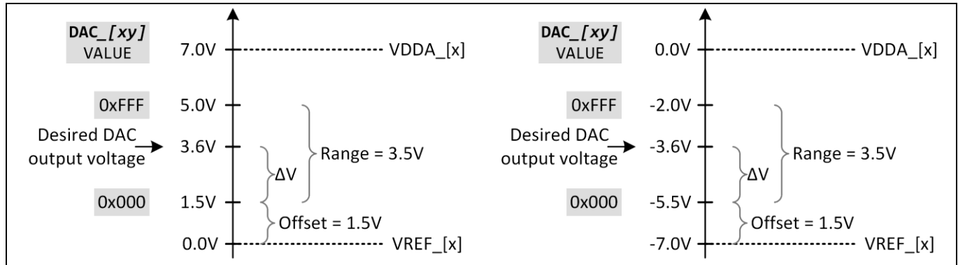
Figure 47 Parameters and their Influence on DAC Output Voltage
