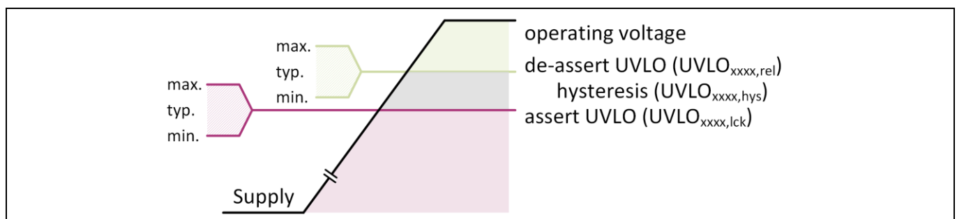
Figure 40 Voltage Monitoring
