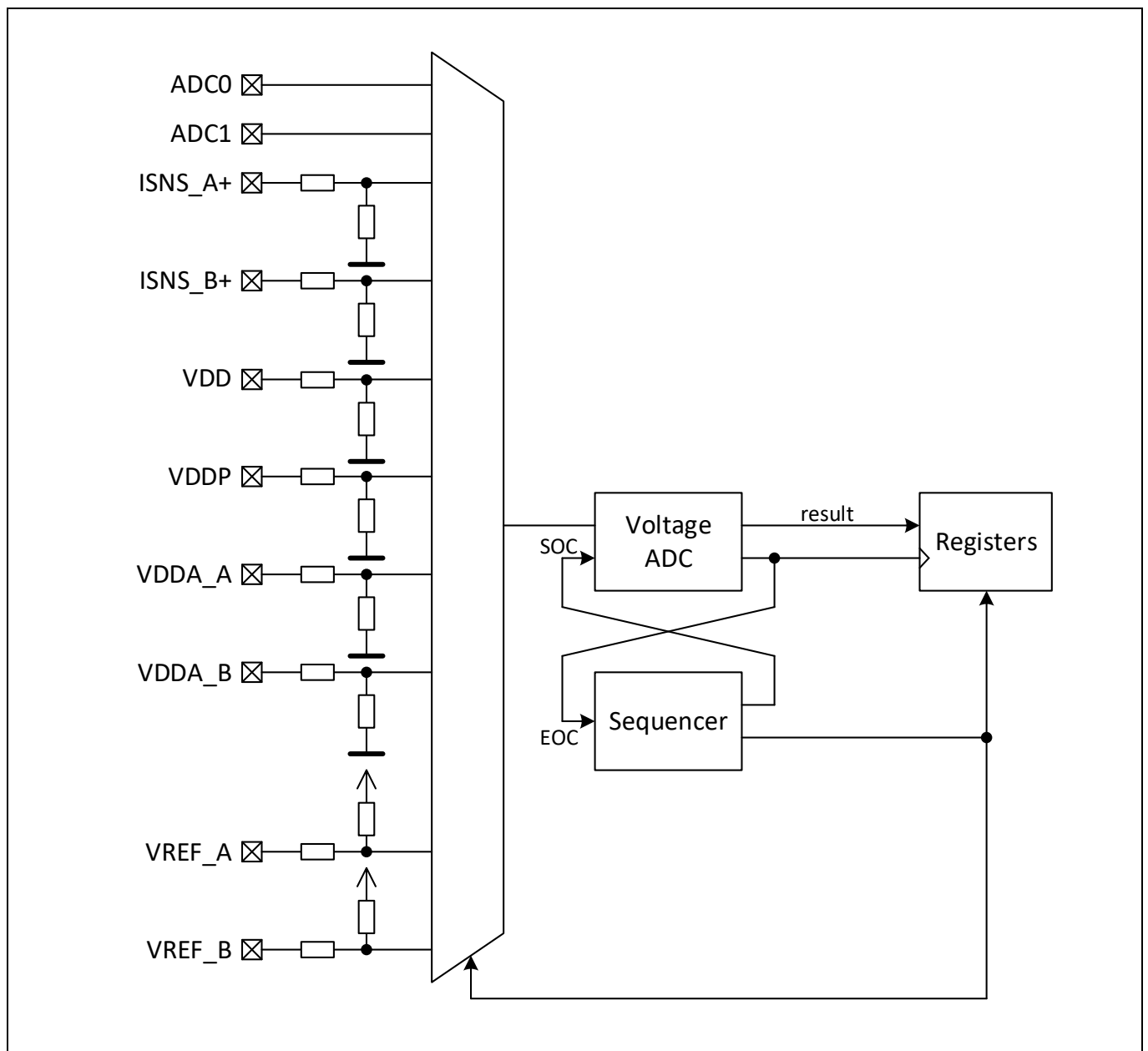
Figure 12 Voltage ADC
