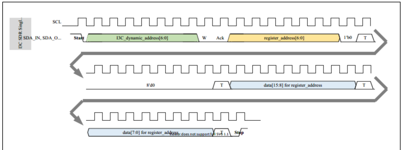
Figure 31 I3C SDR single write
