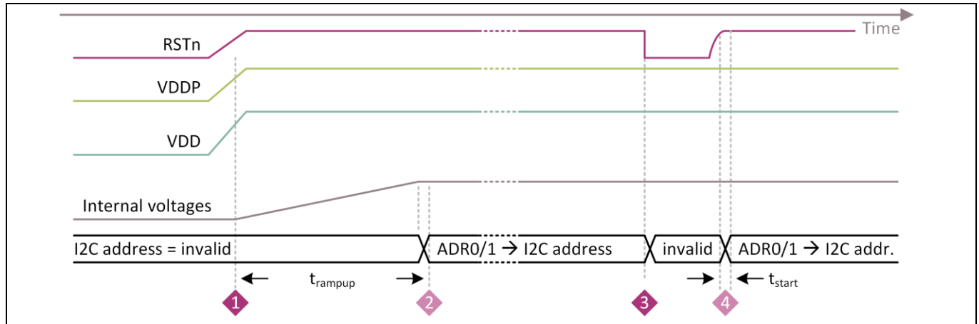
Figure 39 Power-Up and reset Timing
