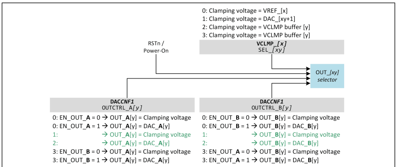
Figure 43 OUT_[xy] Selection
