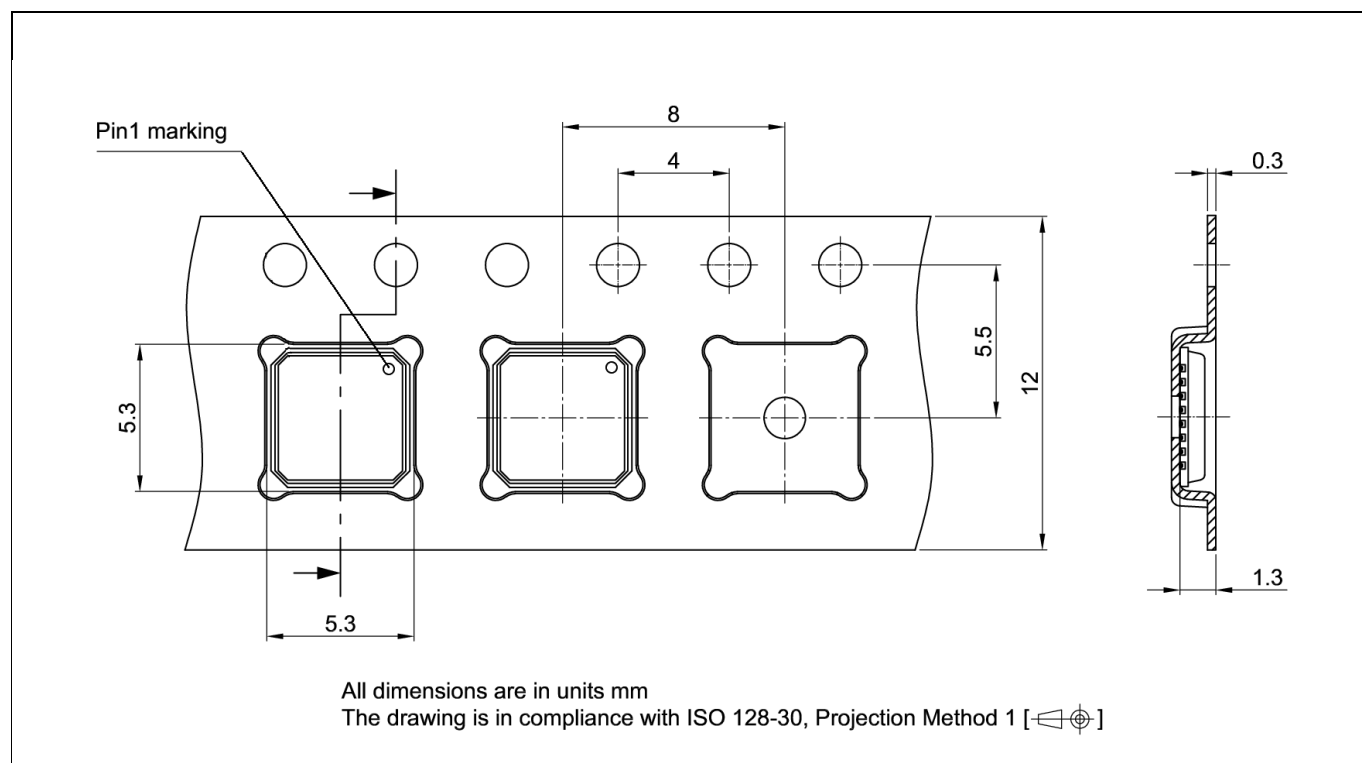
Figure 62 PG-VQFN-32-21 Tape information
