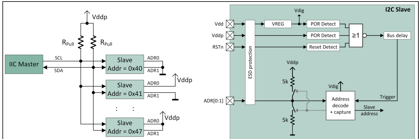
Figure 14 I2C Address Selection
