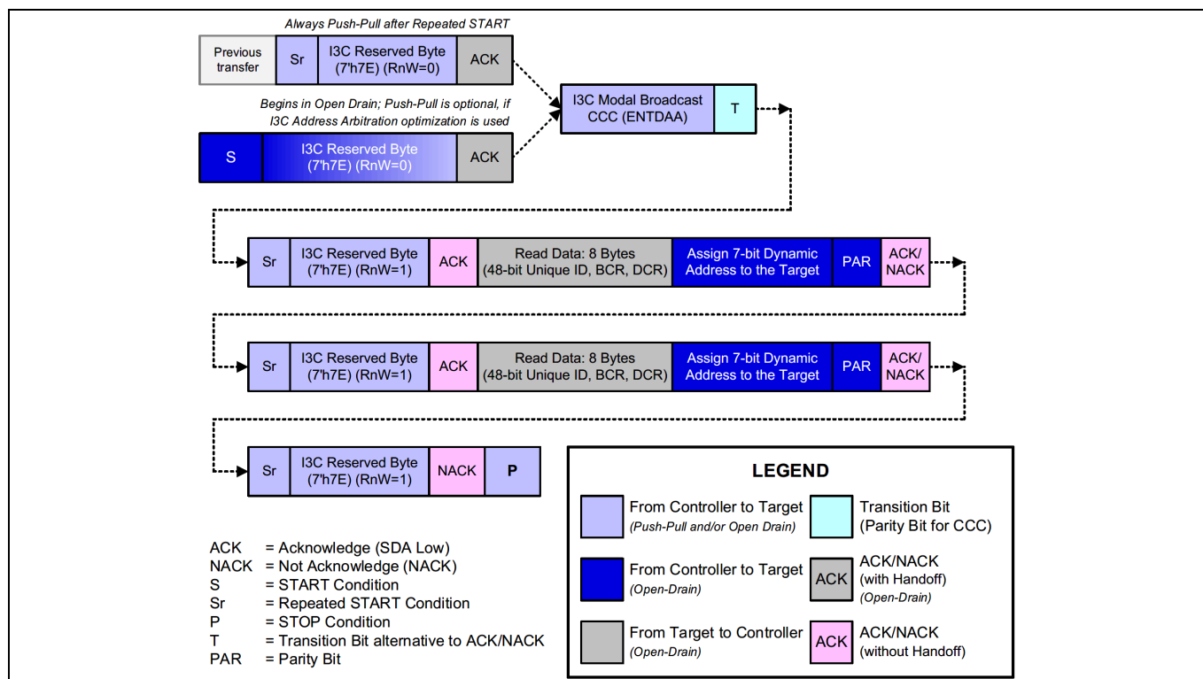
Figure 26 ENTDAAC Command Structure
