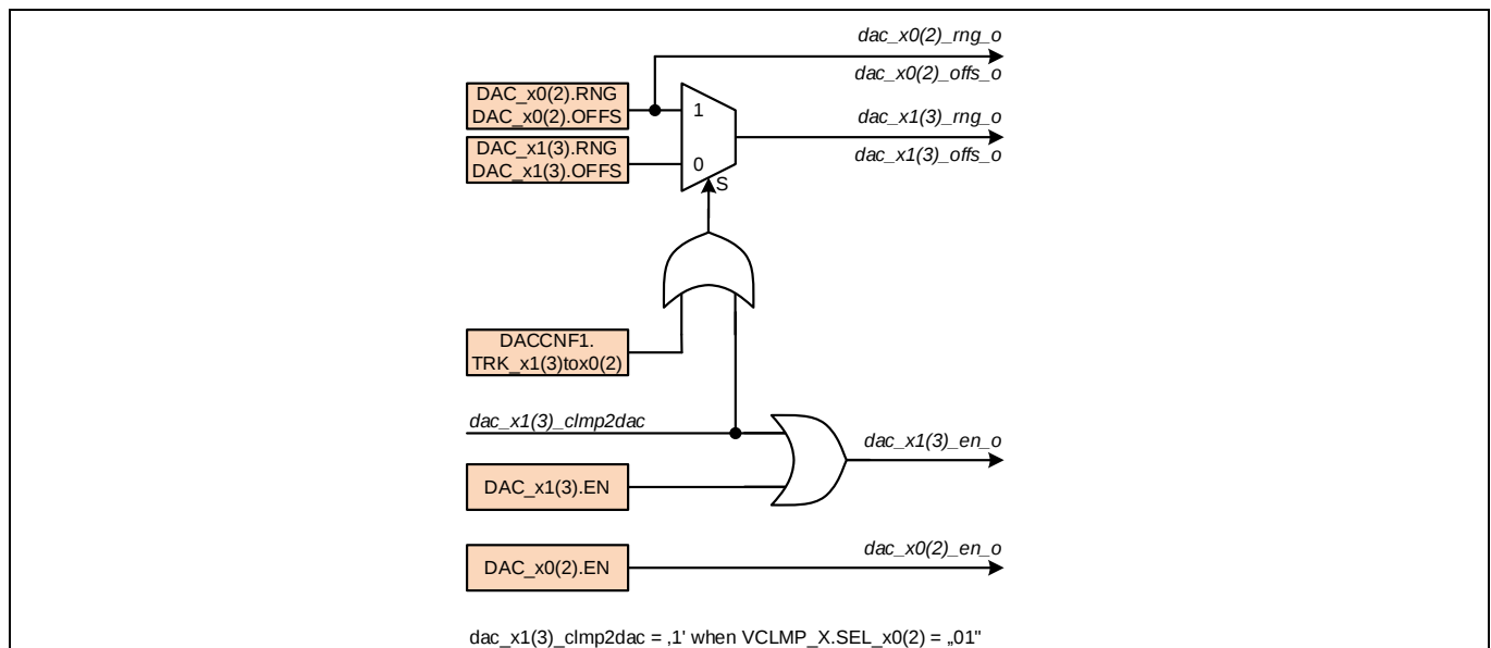
Figure 7 Odd DAC_x1(3) settings in tracking/clamping modes
