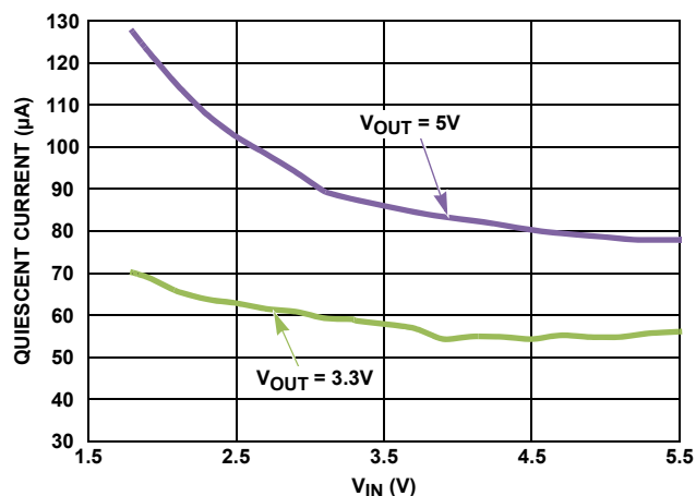
FIGURE 9. QUIESCENT CURRENT vs INPUT VOLTAGE (MODE = HIGH)
