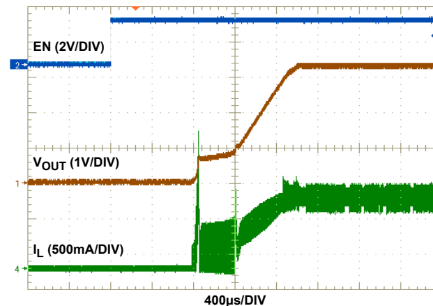
FIGURE 13. SOFT-START ( V_{IN} = 3.6\text{V} , V_{OUT} = 3.3\text{V} , 1A RLOAD)
