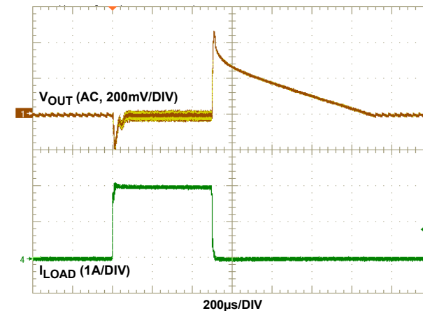
FIGURE 15. 0A TO 2A LOAD TRANSIENT ( V_{IN} = 3.6\text{V} , V_{OUT} = 3.3\text{V} )
