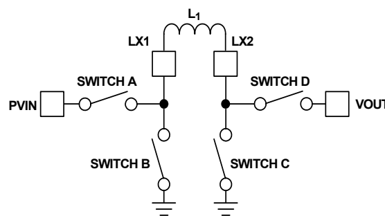
FIGURE 21. BUCK BOOST TOPOLOGY
