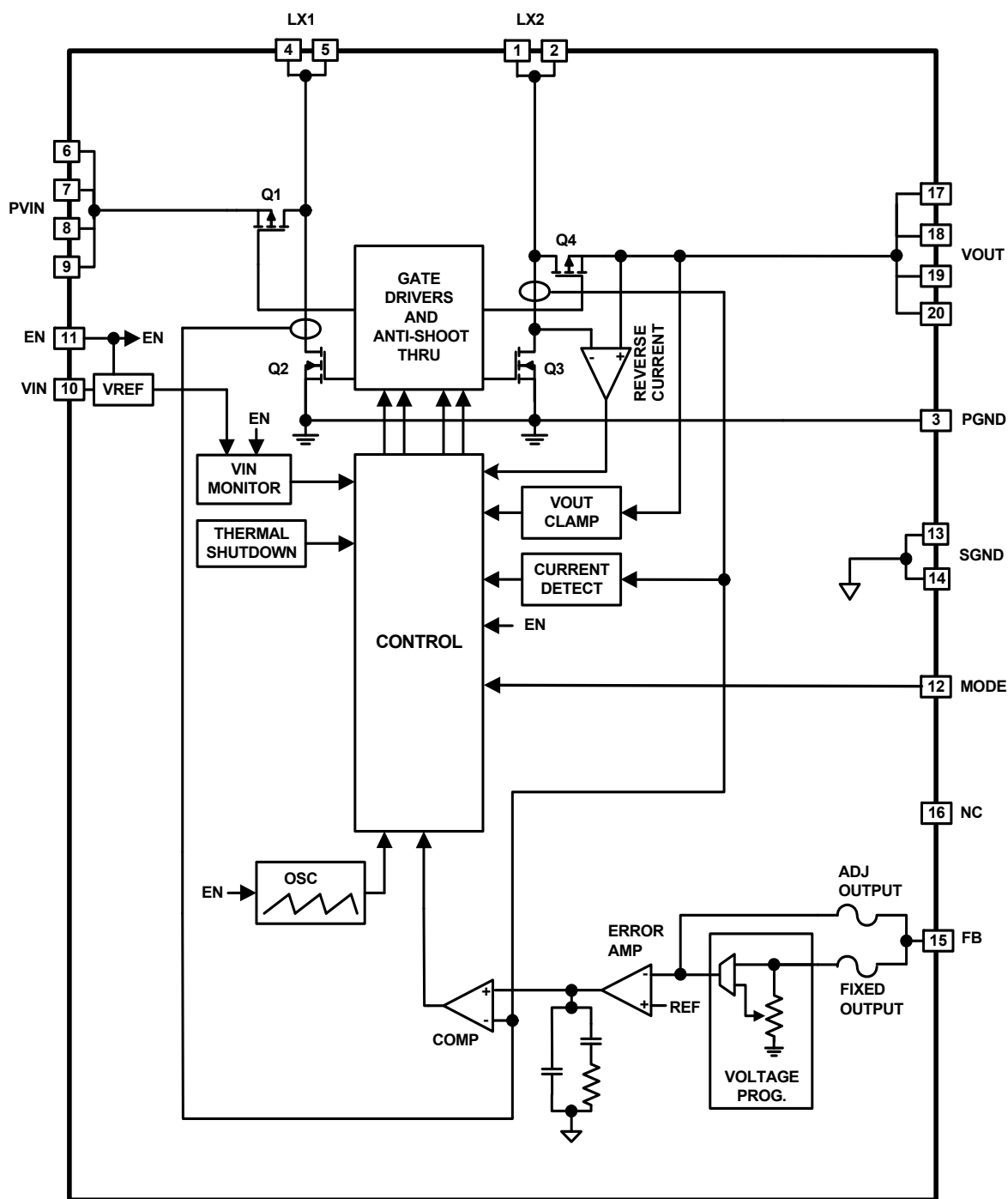
FIGURE 3. BLOCK DIAGRAM
