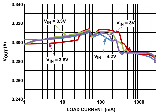
FIGURE 7. OUTPUT VOLTAGE vs LOAD CURRENT ( V_{OUT} = 3.3\text{V} )
