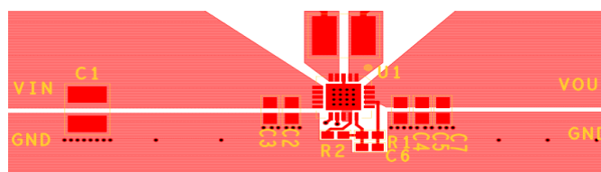
FIGURE 23. RECOMMENDED LAYOUT
