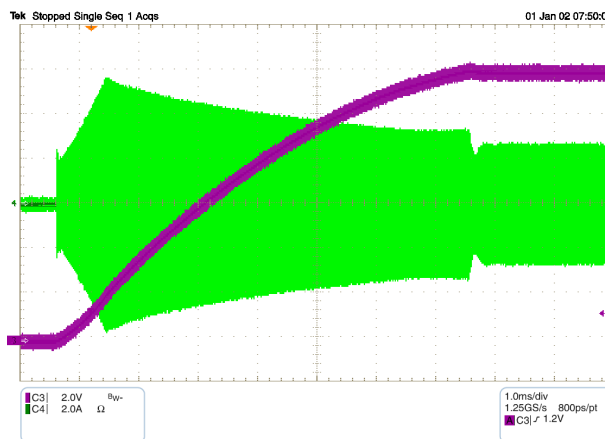
Figure 17. Application Startup with NCP13992 – Primary Current – Green, V_{out} – Magenta
