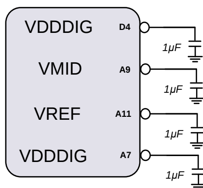
Figure 43: Reference Capacitors
