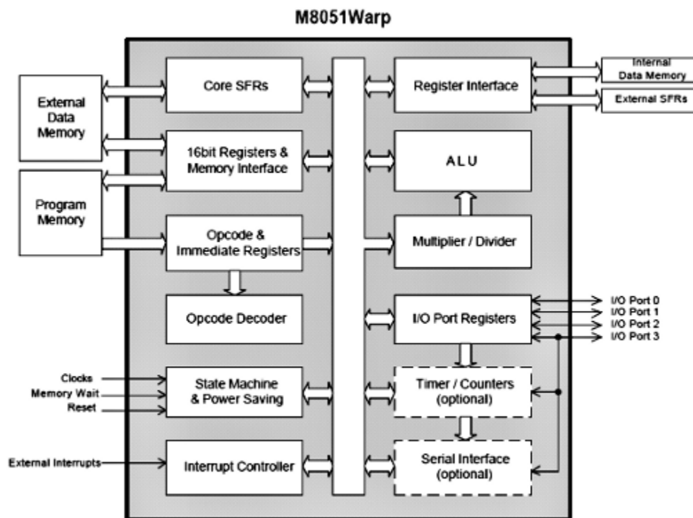
Figure 23. 8051W Core
