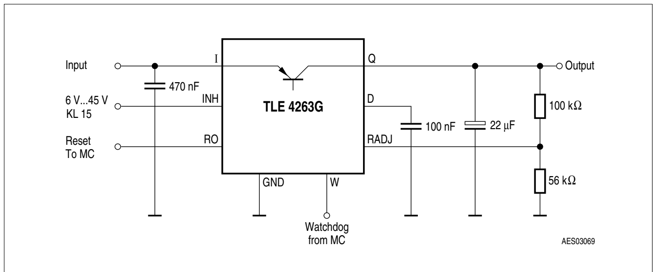
Figure 3 Application circuit
