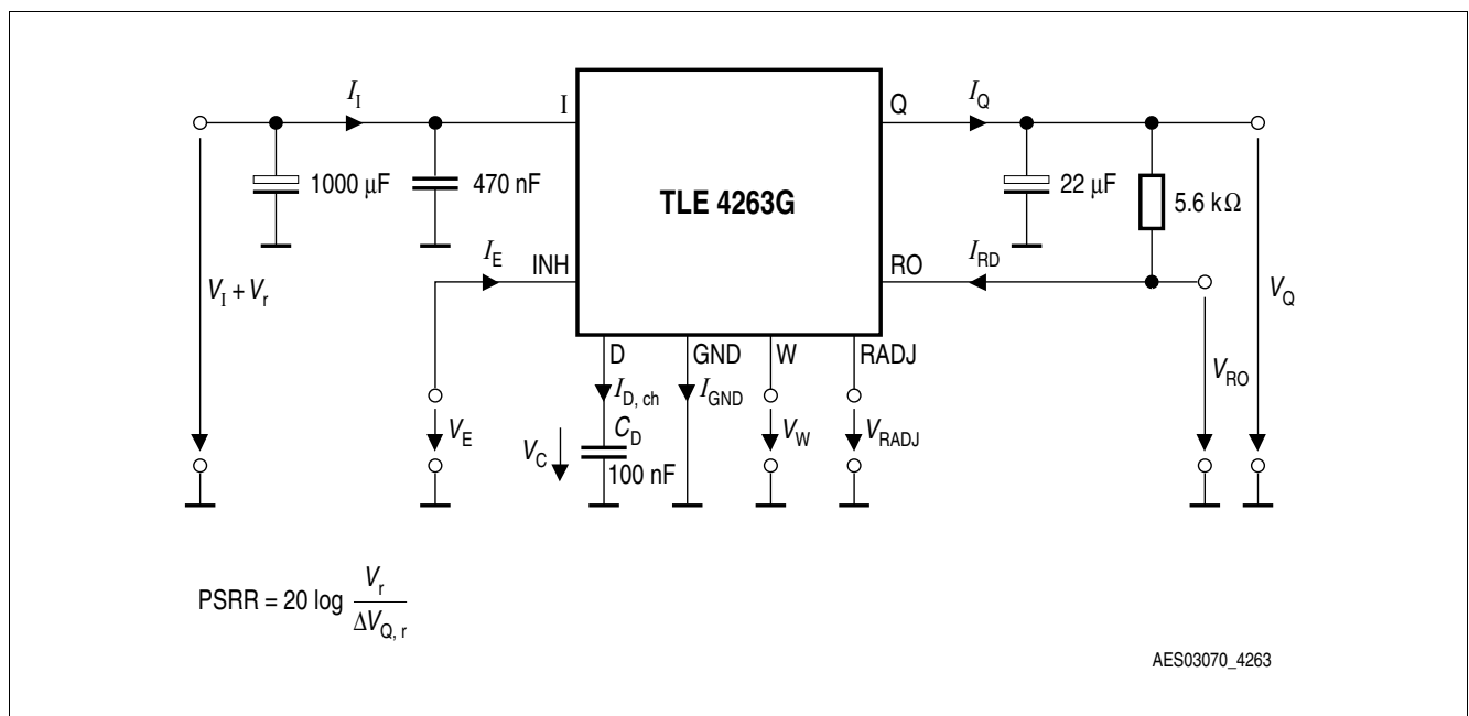
Figure 4 Test circuit
