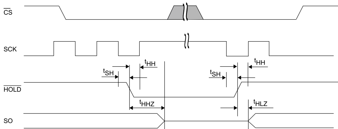
Figure 36. \overline{\text{HOLD}} Timing
