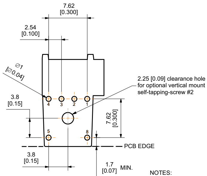
Footprint - TOP VIEW
