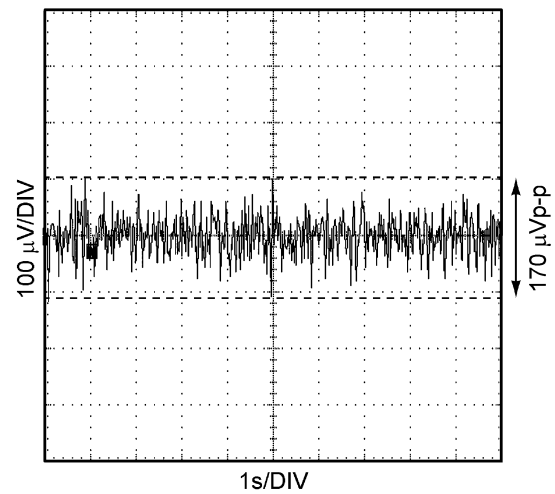
Figure 14. 0.1–10 Hz Noise
