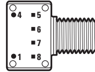
BOTTOM VIEW, HFBR 25x5AZ/BZ
