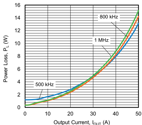
Fig. 8 - Power Loss vs. Output Current
