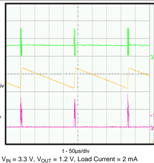
Figure 25. Typical Application (Snooze Mode)
